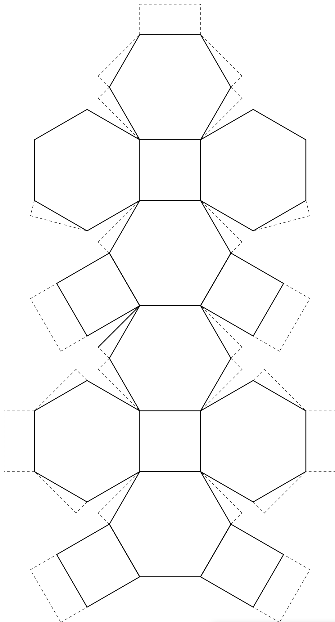
kelvin tetrakaidecahedron
